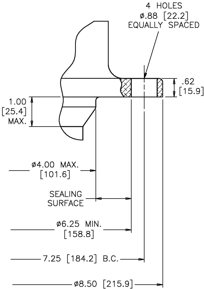
MOUNTING FLANGE DETAIL
