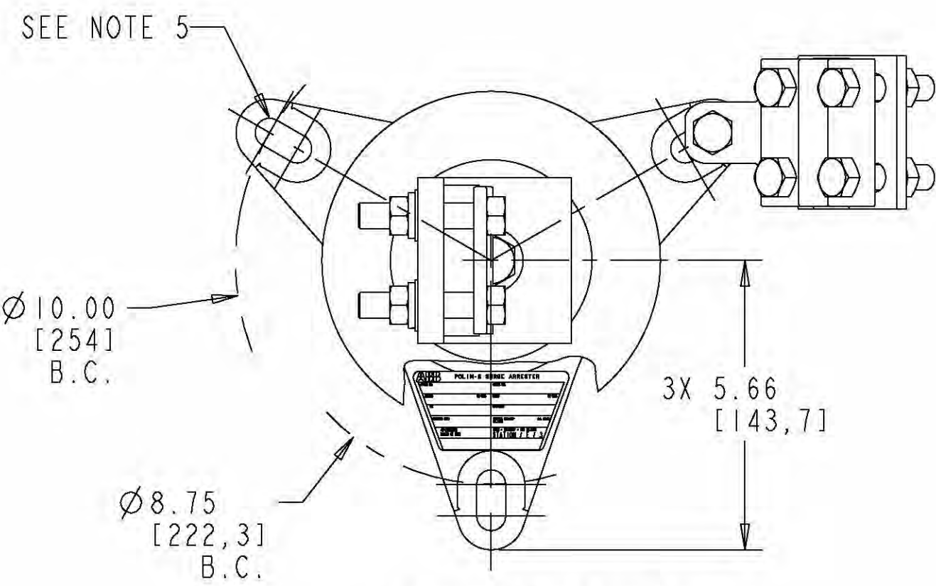
DETAIL B (ENLARGED) SCALE 0.500 GROUND TERMINAL (GALVANIZED) (CAN BE ATTACHED TO ANY LUG)
