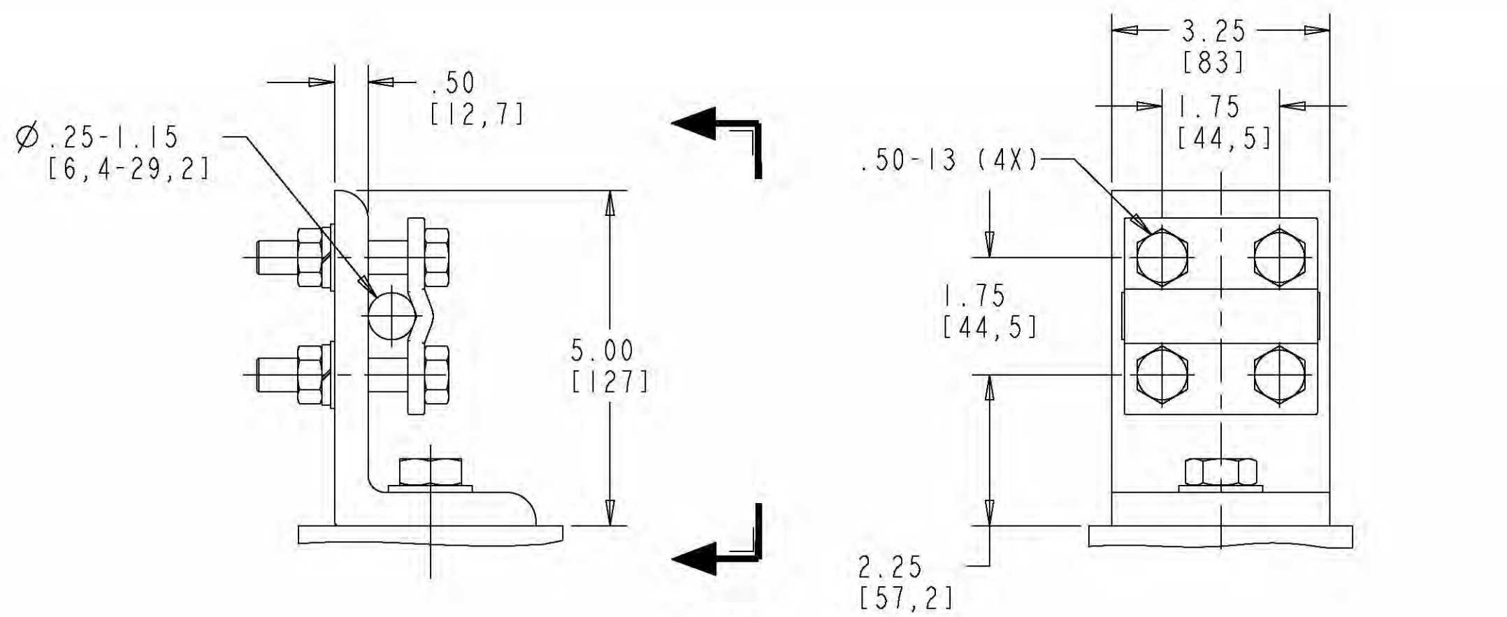
DETAIL A (ENLARGED) SCALE 0.500 LINE TERMINAL (ALUMINUM) (CAN BE ADJUSTED TO ANY ANGLE)
